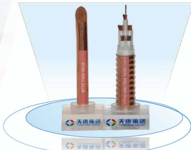
Mineral-insulated cable
